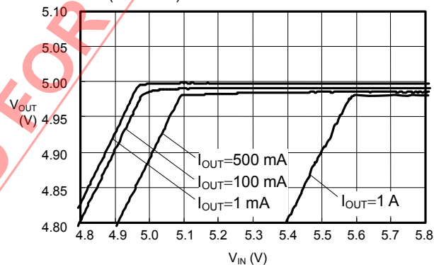
V_{IN} - V_{OUT} S-816A50AMC ( T_a=25^\circ\text{C} )
