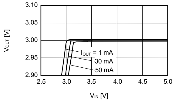
S-1323B30 (Ta=25°C)
