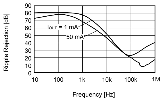
S-1200B30 (Ta=+25°C)
