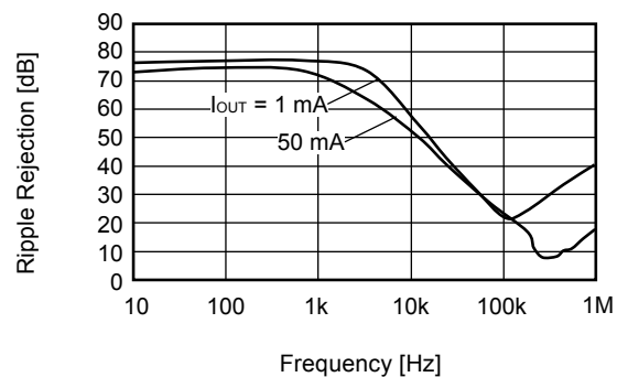
S-1200B50 (Ta=+25°C)
