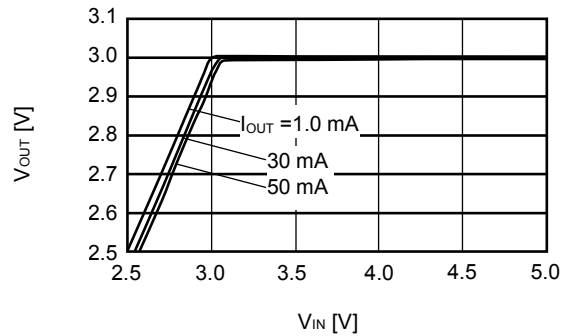
S-1200B30 (Ta=+25°C)
