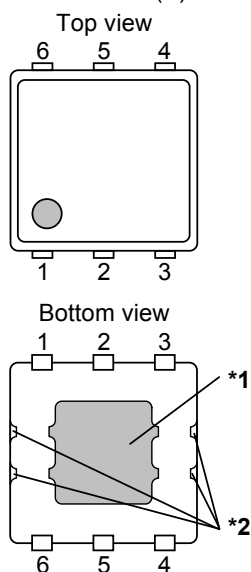
6-Pin HSON(A)
