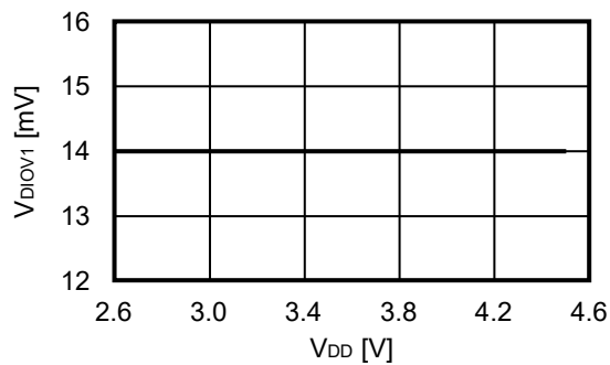
2.5 V_{DIOV1} - V_{DD}
