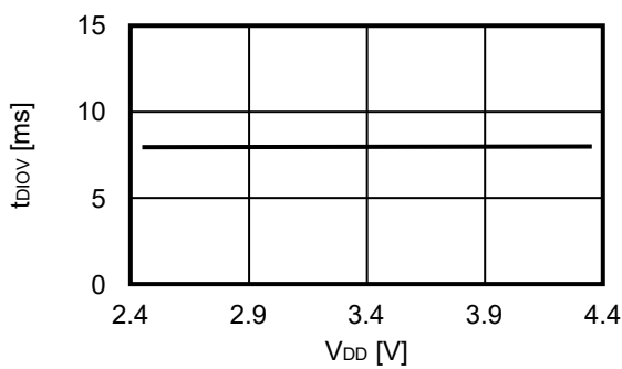
3.3 t_{DIOV} - V_{DD}
