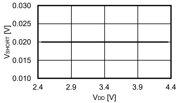
2.7 V_{SHORT} - V_{DD}
