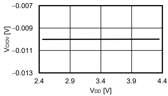
2.9 V_{CIOV} - V_{DD}
