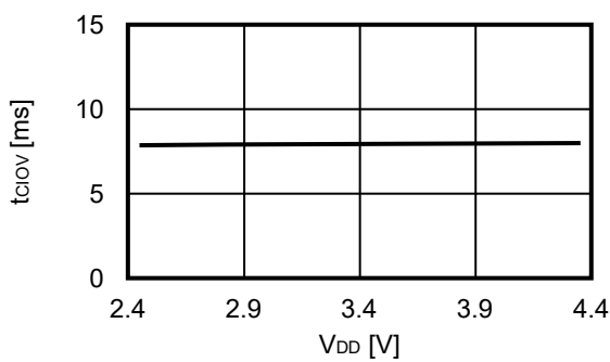
3.7 t_{CIOV} - V_{DD}
