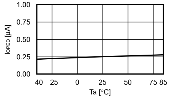
1.2 I_{OPED} - T_a
