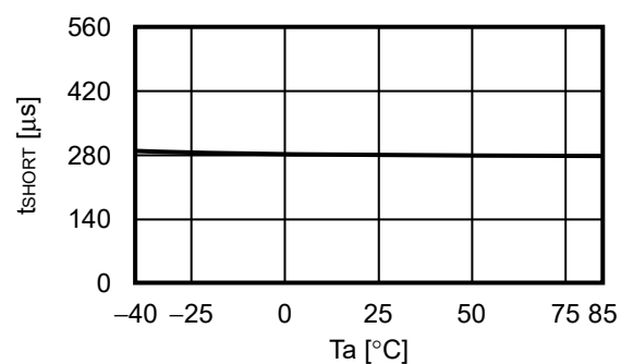
3.8 t_{SHORT} - T_a
