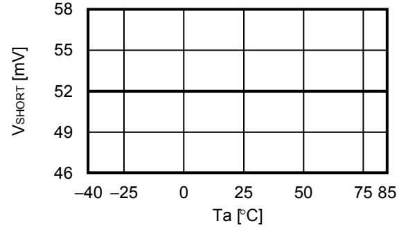
2. 10 V_{SHORT} - T_a
