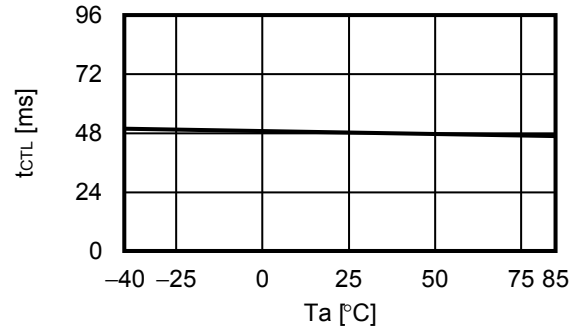
3.12 t_{CTL} - T_a
