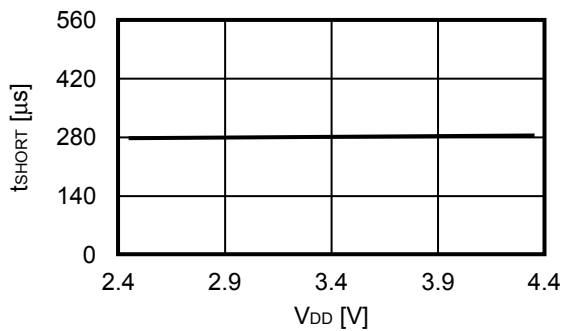
3.7 t_{SHORT} - V_{DD}
