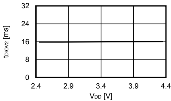
3.5 t_{DIOV2} - V_{DD}
