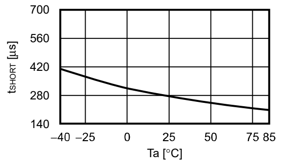
3.6 t_{SHORT} - T_a
