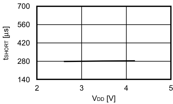
3.5 t_{SHORT} - V_{DD}
