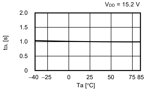
3.2 t_{DL} - T_a
