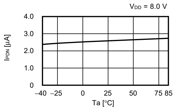
2.2 I_{PDN} - T_a
