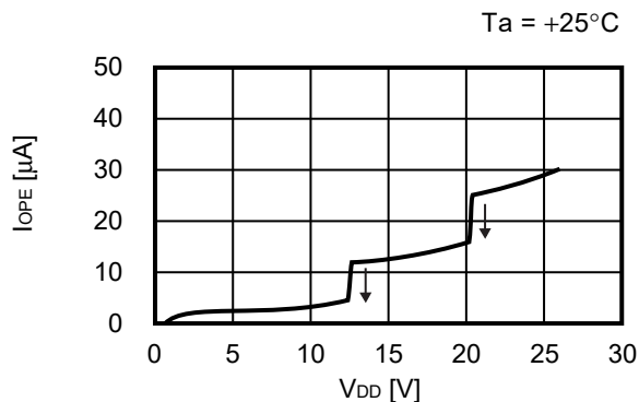
2.3 I_{OPE} - V_{DD}
