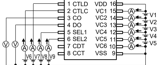
図9 測定回路6
