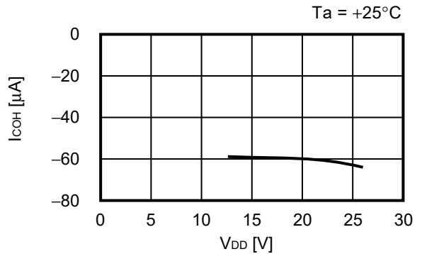
4.2 I_{CO(H)} - V_{DD}
