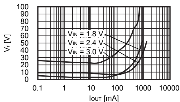
Condition 8 S-8366ABBBA ( V_{OUT(S)} = 3.3 \text{ V} )
