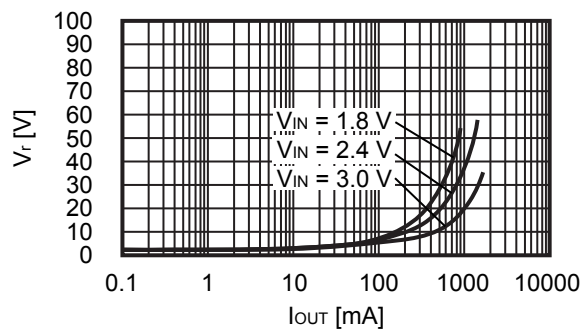
Condition 6 S-8365ABBBA ( V_{OUT(S)} = 3.3 \text{ V} )
