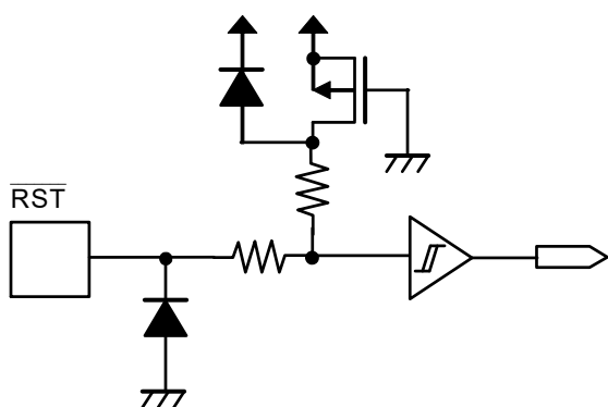
Figure 5 \overline{\text{RST}} Pin
