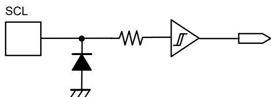
Figure 3 SCL Pin
