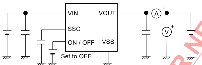
Figure 8 Test Circuit 6
