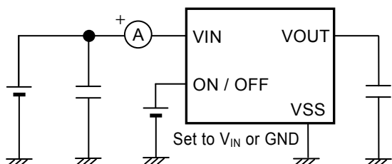
Figure 9 Test Circuit 2
