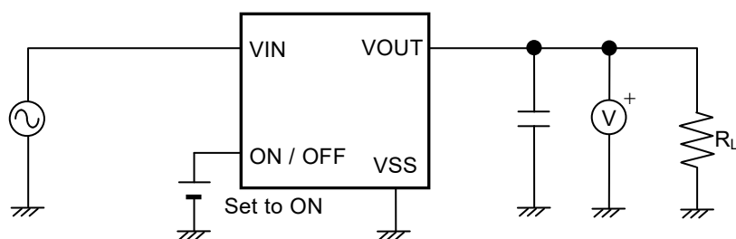
Figure 10 Test Circuit 5
