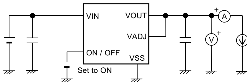
Figure 11 Test Circuit 6
