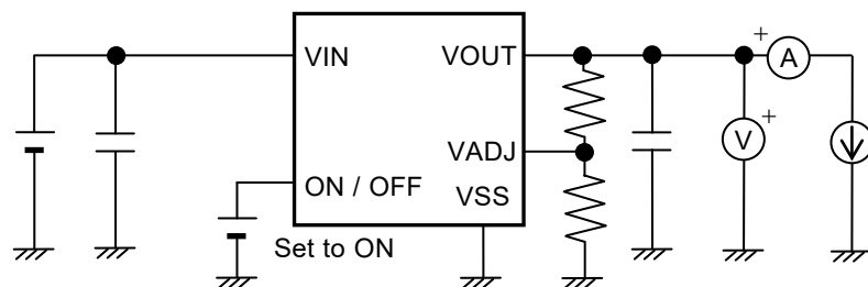
Figure 16 Test Circuit 11
