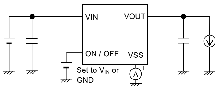
Figure 7 Test Circuit 2
