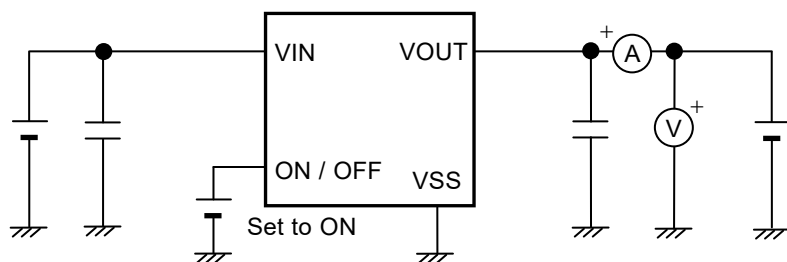
Figure 8 Test Circuit 3
