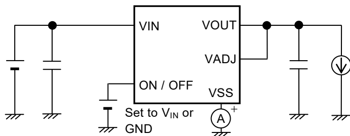
Figure 12 Test Circuit 7
