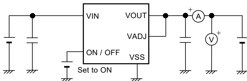
Figure 13 Test Circuit 8
