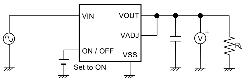
Figure 15 Test Circuit 10
