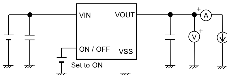
Figure 6 Test Circuit 1
