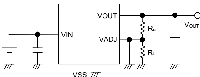
Figure 21 When The VADJ Pin Is In The Short State To V_{SS}
