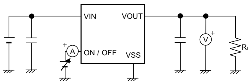
Figure 9 Test Circuit 4
