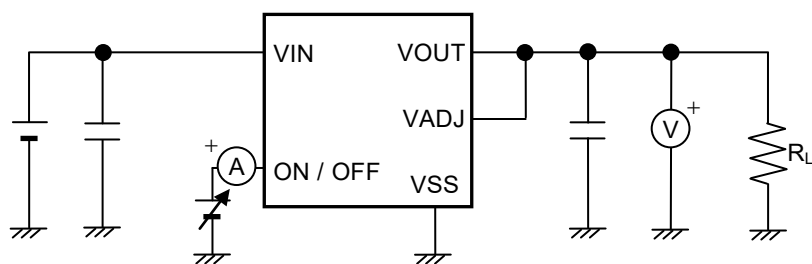
Figure 14 Test Circuit 9
