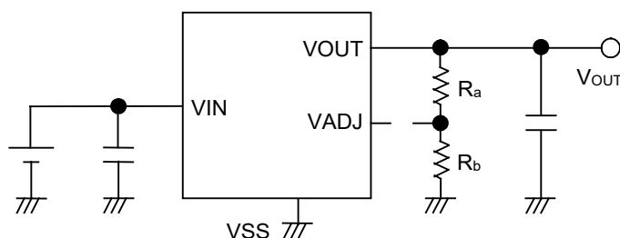
Figure 20 When The VADJ Pin Is In The Open State
