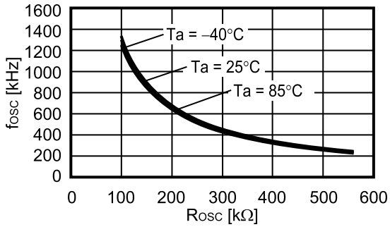
f_{OSC} vs. R_{OSC} ( V_{IN} = 3.3\text{ V} )
