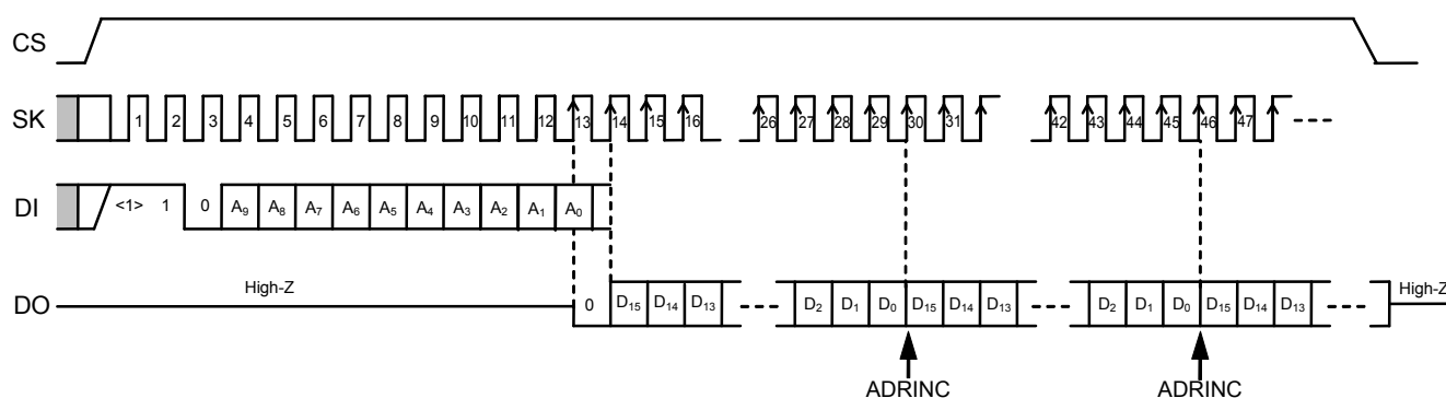
Figure 5 Read Timing
