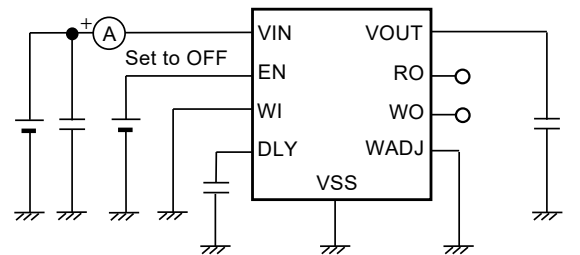
Figure 32 Test Circuit 10
