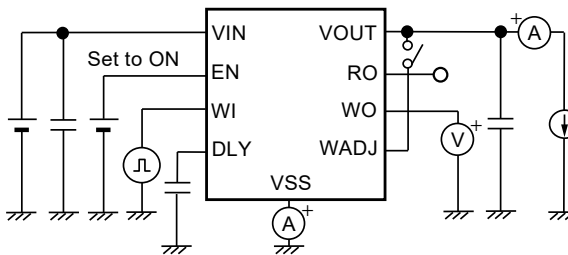
Figure 31 Test Circuit 9
