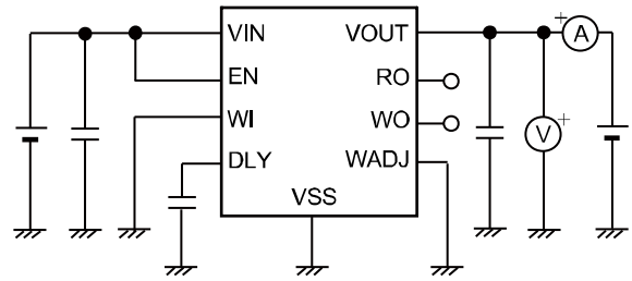
Figure 24 Test Circuit 2
