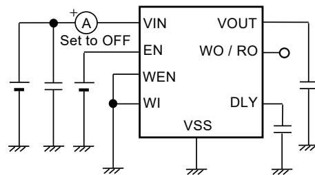
Figure 22 Test Circuit 10
