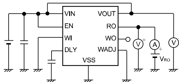
Figure 28 Test Circuit 6
