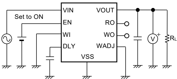
Figure 25 Test Circuit 3
