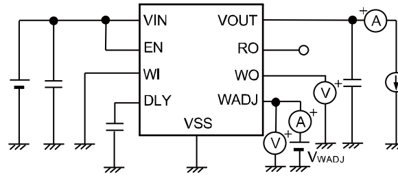
Figure 30 Test Circuit 8
