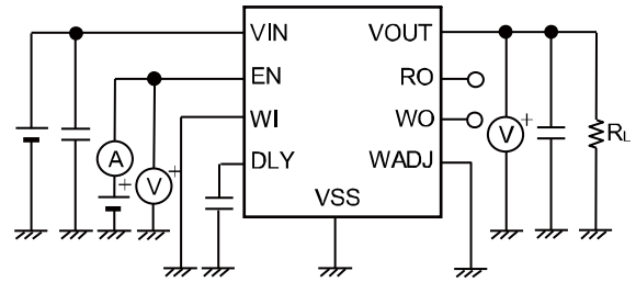
Figure 26 Test Circuit 4
