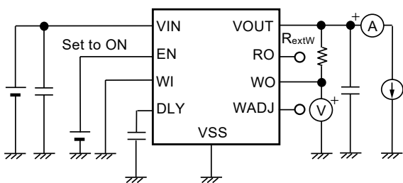
Figure 29 Test Circuit 7
