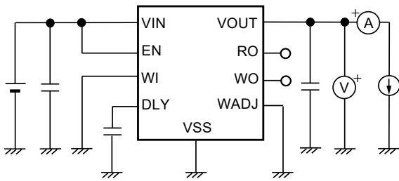
Figure 23 Test Circuit 1
