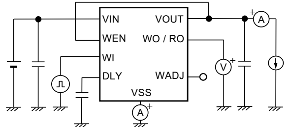
Figure 21 Test Circuit 10
