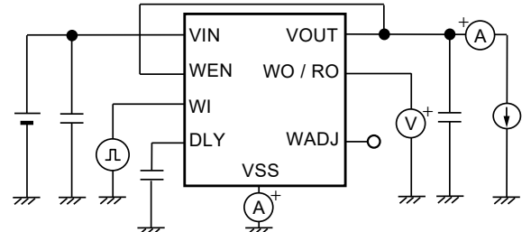
Figure 19 Test Circuit 10
