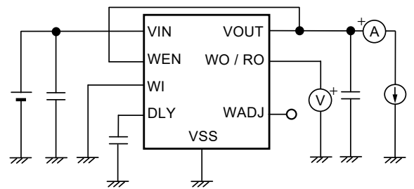
Figure 15 Test Circuit 6
