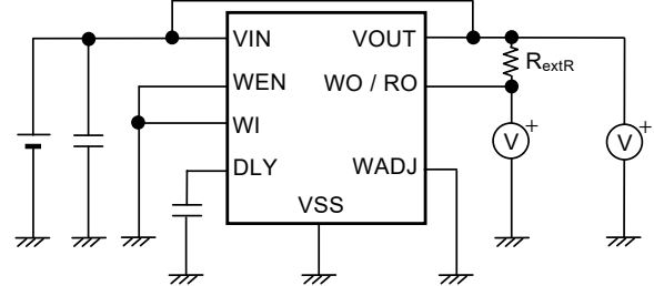
Figure 13 Test Circuit 4
