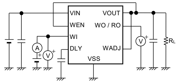
Figure 17 Test Circuit 8
