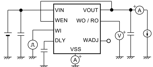
Figure 19 Test Circuit 10
