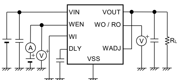
Figure 18 Test Circuit 9
