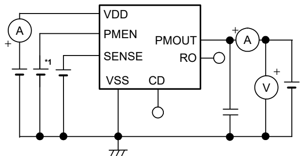
Figure 10 Test Circuit 6
