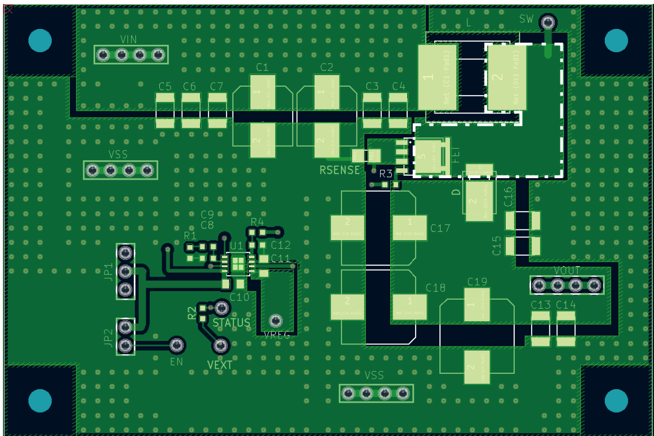
Figure 13 Reference Board Pattern
