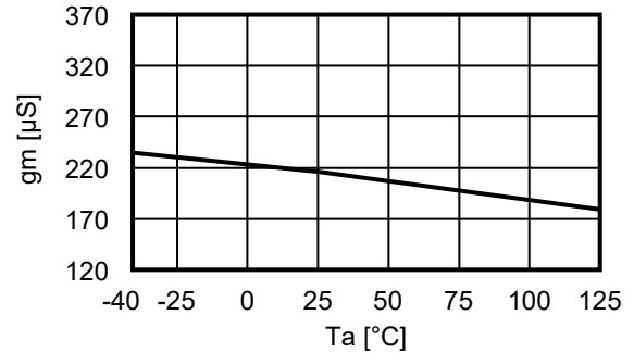
2. 13 Error amplifier transconductance ( g_m ) vs. Temperature ( T_a )
