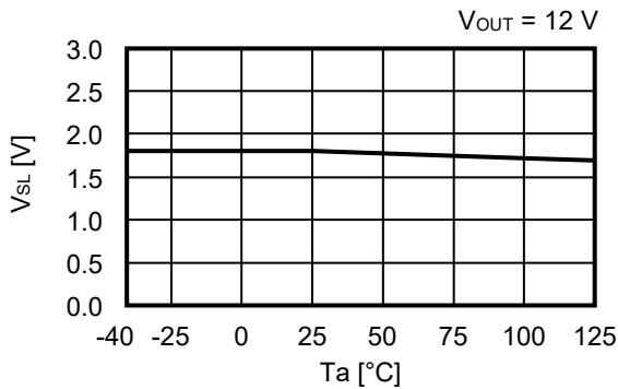
2. 12 Low level input voltage ( V_{SL} ) vs. Temperature ( T_a )
