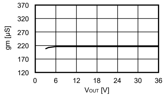
1.9 Error amplifier transconductance ( g_m ) vs. Output voltage ( V_{OUT} )
