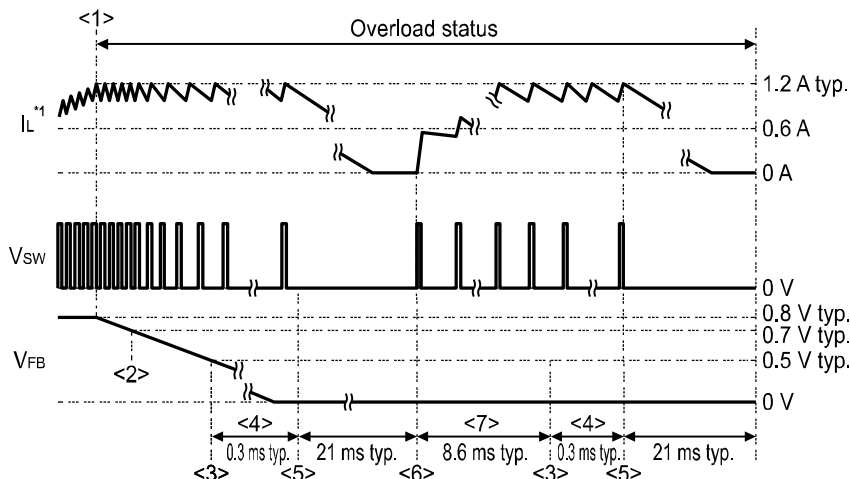
*1. Inductor current
