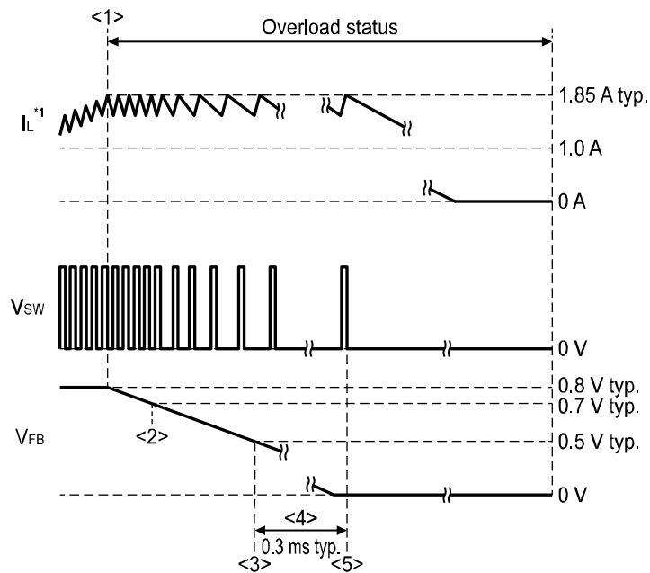
*1. Inductor current
