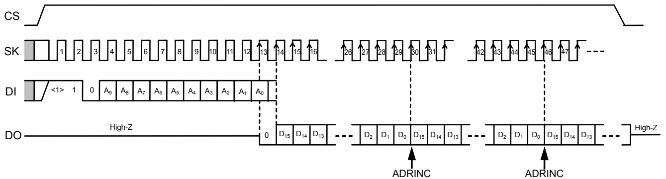
Figure 5 Read Timing
