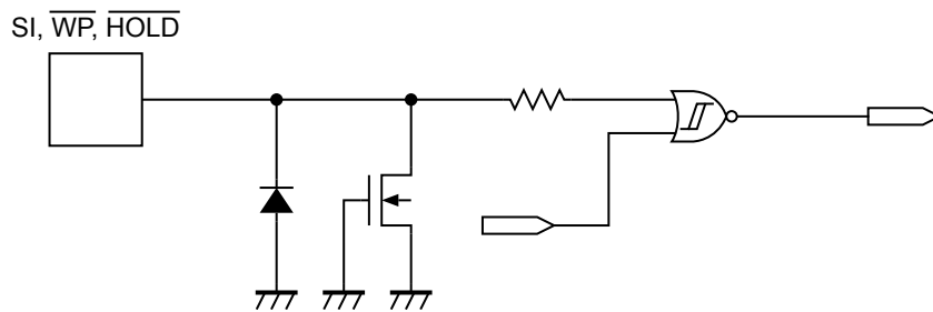
Figure 25 SI, \overline{WP} , \overline{HOLD} Pins
