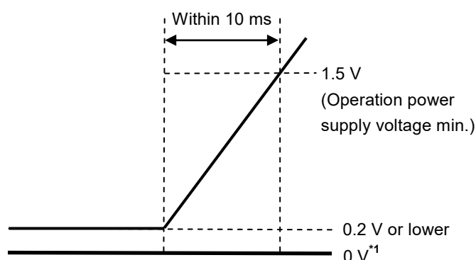
Figure 26 How to Raise the Power Supply Voltage
