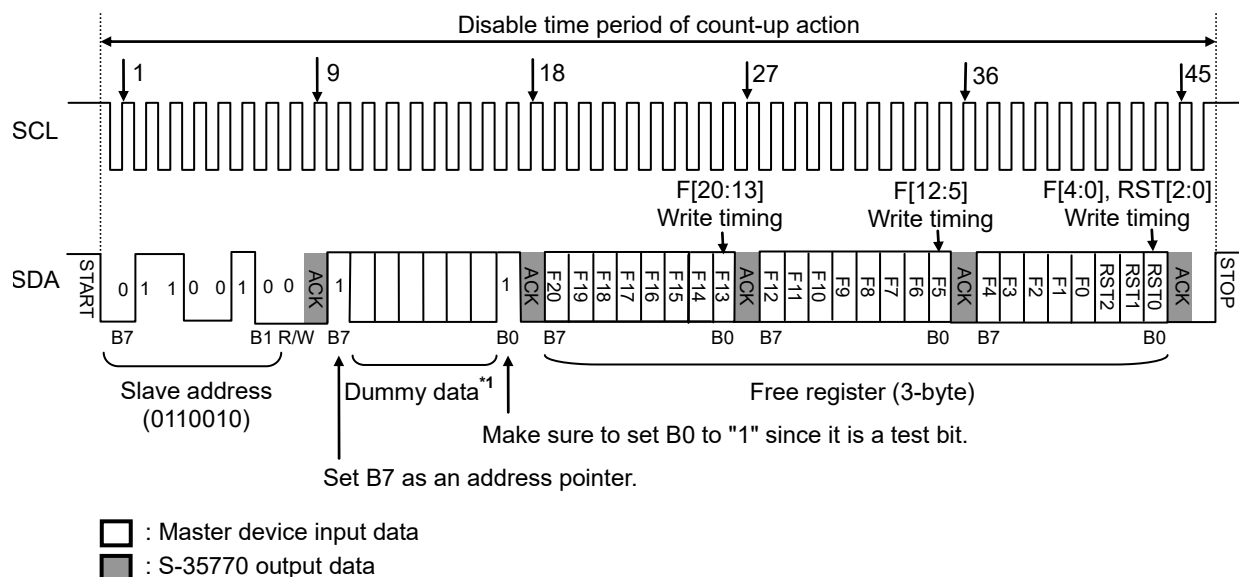
Figure 23 Write Timing of Free Register
