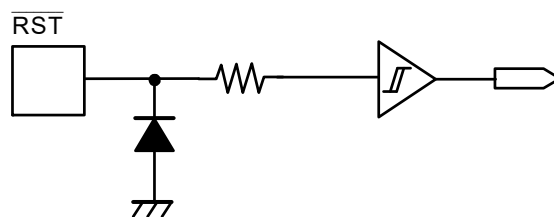
Figure 6 \overline{\text{RST}} Pin (Without Pull-up Resistor)
