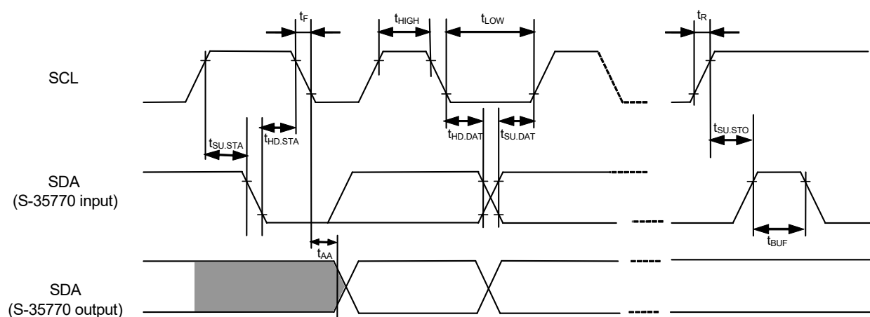
Figure 10 Bus Timing
