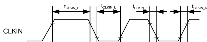
Figure 12 CLKIN Pin Clock Timing
