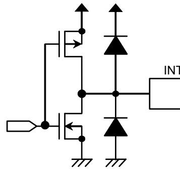
Figure 7 INT Pin (CMOS Output)
