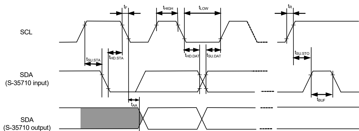
Figure 10 Bus Timing
