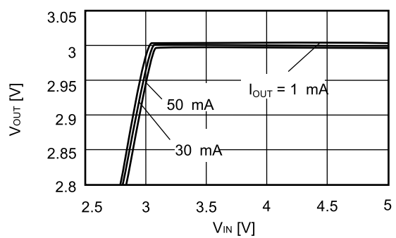
S-1165B30 ( T_a = 25^\circ\text{C} )
