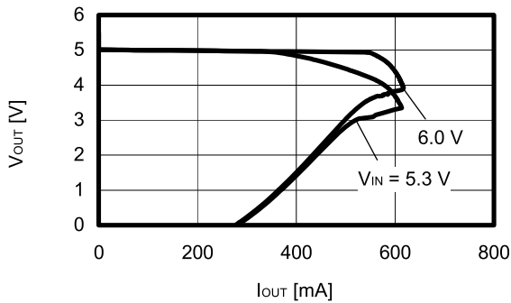
S-1165B50 ( T_a = 25^\circ\text{C} )
