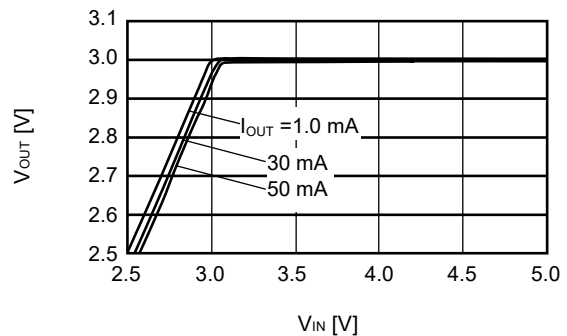
S-1200B30 ( T_a=+25^\circ\text{C} )
