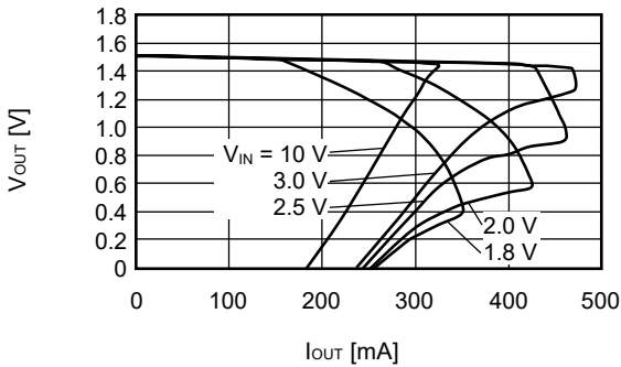
S-1200B50 ( T_a=+25^\circ\text{C} )
