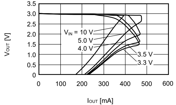
S-1200B30 ( T_a=+25^\circ\text{C} )
