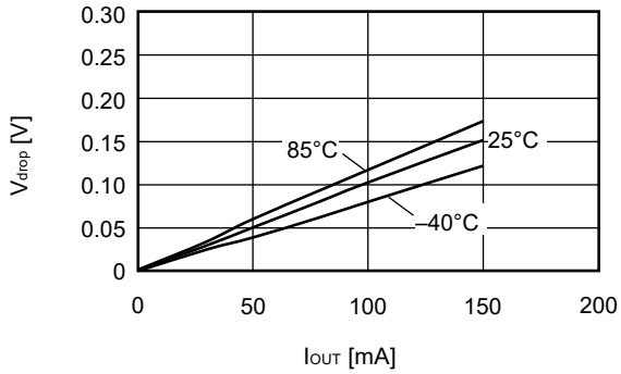
S-1200B50
