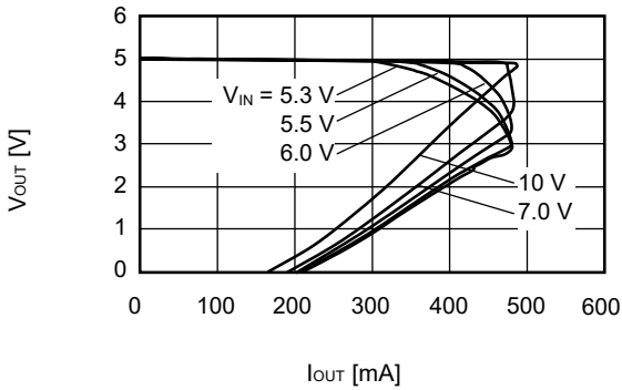
S-1200B50 ( T_a=+25^\circ\text{C} )
