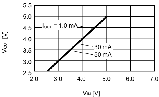
S-1200B50 ( T_a=+25^\circ\text{C} )
