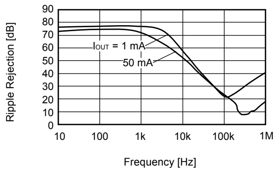
S-1200B50 (Ta=+25°C)
