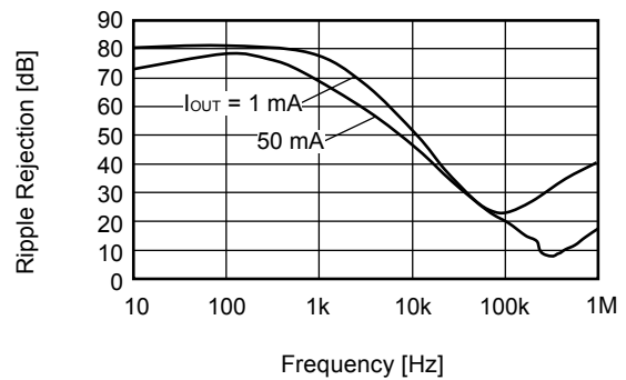
S-1200B30 (Ta=+25°C)
