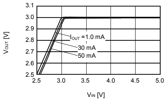
S-1200B30 (Ta=+25°C)
