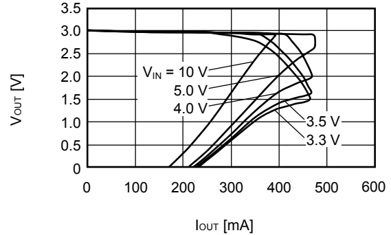
S-1200B30 (Ta=+25°C)
