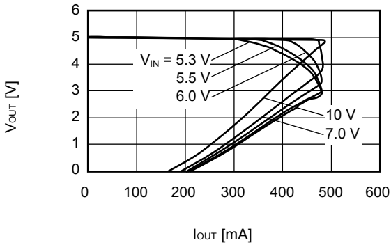
S-1200B50 (Ta=+25°C)
