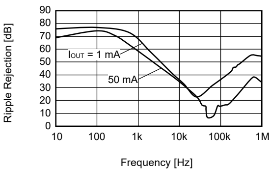
S-1200B50 (Ta=+25°C)
