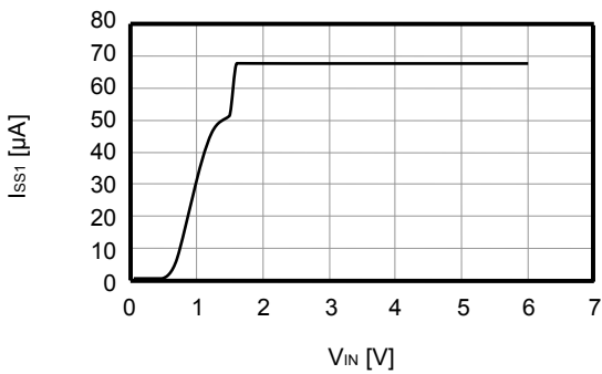
S-1170B50 ( T_a=25^\circ\text{C} )
