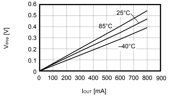
S-1170B30
