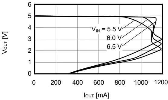
S-1170B50 (Ta=25°C)
