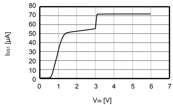
S-1170B30 ( T_a=25^\circ\text{C} )
