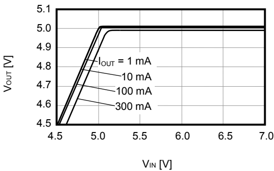
S-1170B50 (Ta=25°C)
