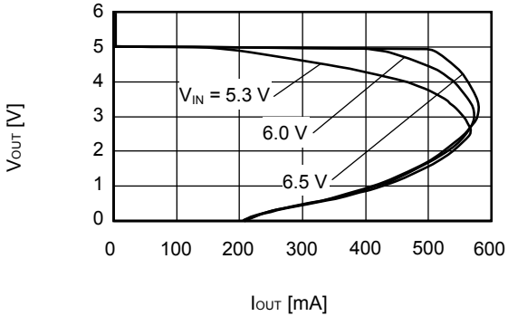
S-1112B50 (Ta=25°C)
