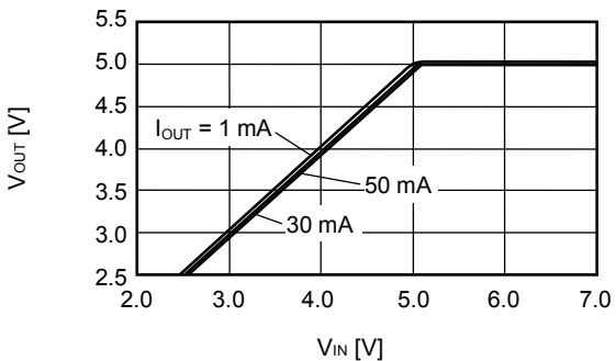
S-1112B50 (Ta=25°C)
