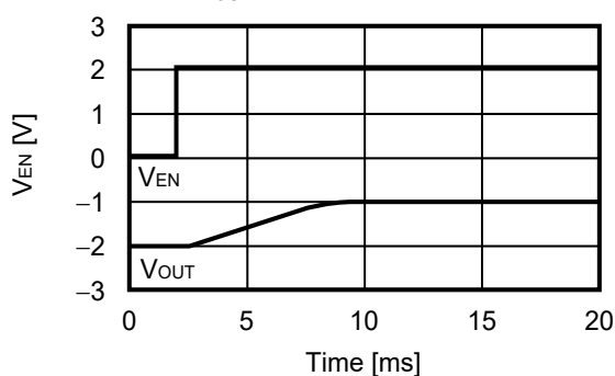
4.2.1 I_{OUT} = 1\text{ mA}
