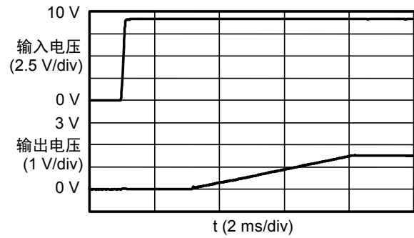
S-8533A33AFT ( V_{IN}: 0\text{ V} \rightarrow 9.0\text{ V} )
