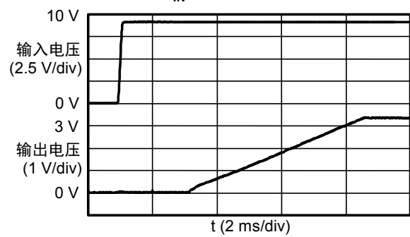
S-8533A50AFT ( V_{IN}: 0\text{ V} \rightarrow 9.0\text{ V} )
