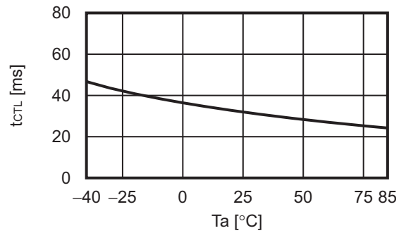
3.12 t_{CTL} - T_a
