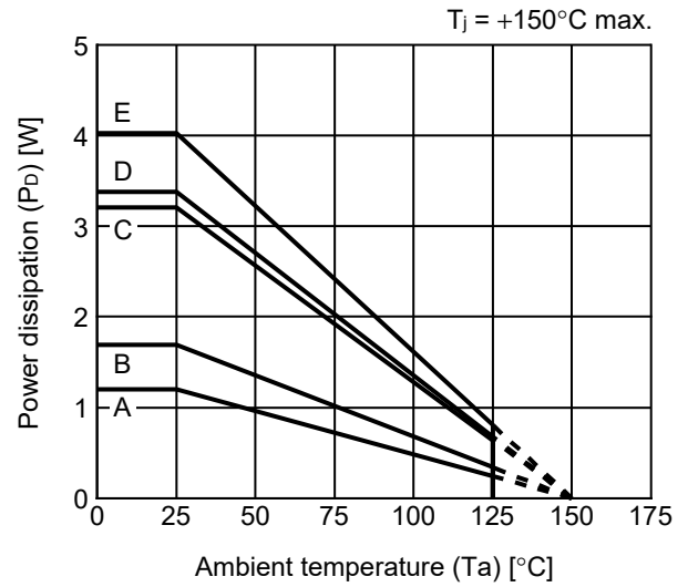
HSOP-8A
