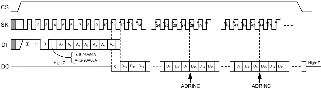
图7 读出定时 (S-93A56A, S-93A66A)
