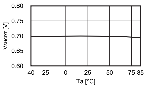
2. 19 V_{SHORT} - T_a
