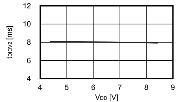
2.14 t_{DIOV2} - V_{DD}
