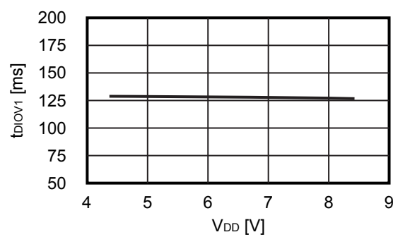
2.11 t_{DIOV1} - V_{DD}
