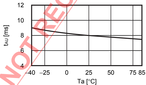
2.7 t_{AU} - T_a
