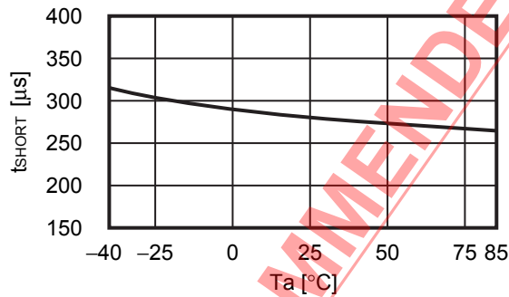
2. 21 t_{SHORT} - T_a
