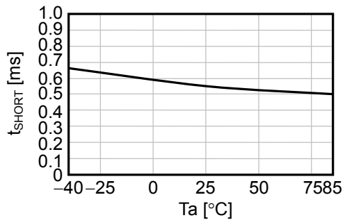
2. 15 t_{SHORT} - T_a
