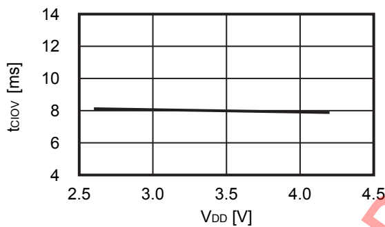
2. 11 t_{CIOV} - V_{DD}
