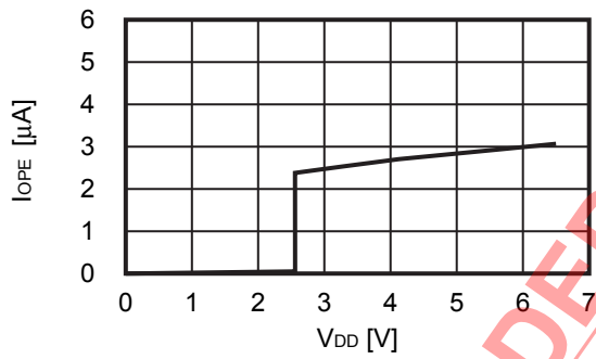
1.3 I_{OPE} - V_{DD}
