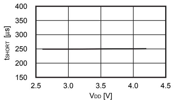
2. 14 t_{SHORT} - V_{DD}
