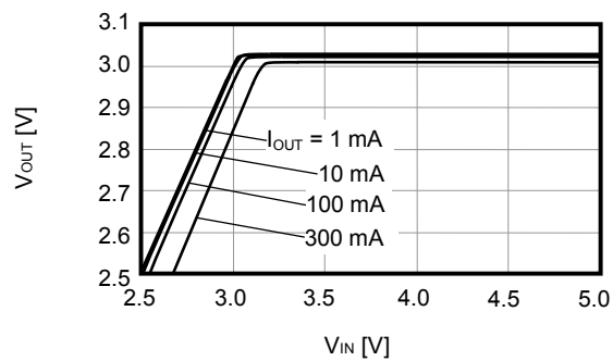
S-1170B30 (Ta=25°C)
