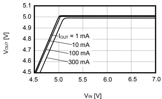
S-1170B50 (Ta=25°C)
