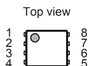
図3 S-35391A-I8T1U
