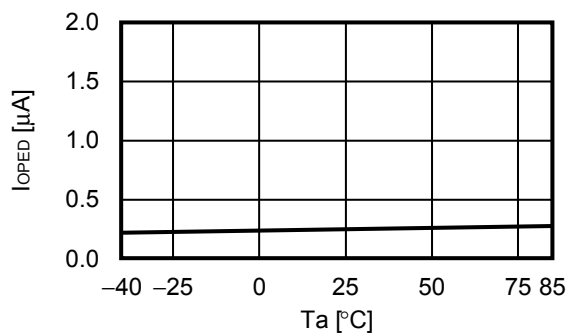
1.3 I_{OPED} - T_a
