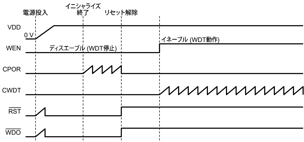
図36 WEN端子 = "L" → "H"
