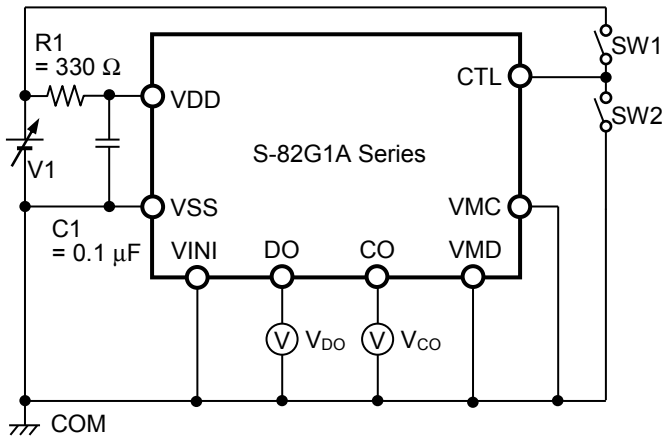
Figure 3 Test Circuit 1
