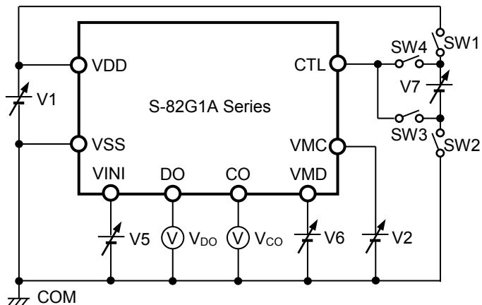
Figure 4 Test Circuit 2
