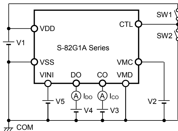
Figure 6 Test Circuit 4
