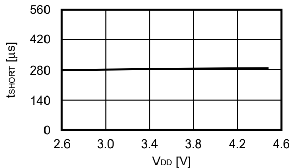
3.7 t_{SHORT} - V_{DD}
